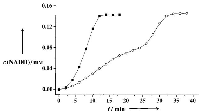
Figure 2. Influence of \text{O}_2 on the indirect electrochemical regeneration of NADH; [\text{Cp}^*\text{Rh}(\text{bpy})\text{Cl}]\text{Cl} (0.1 mM in 50 mM potassium phosphate buffer pH 7.5) (■ no air insertion; ○ air input 10 \text{ cm}^3 \text{ min}^{-1} until t = 25 \text{ min} ).
