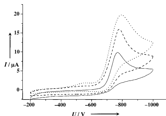
Figure 1. Catalytic effects of [\text{Cp}^*\text{Rh}(\text{bpy})\text{Cl}]\text{Cl} ( 5 \times 10^{-4} \text{ M} in 0.1 M TRIS/HCl buffer pH 7.5; TRIS = tris(hydroxymethyl)aminomethane) in the presence of various concentrations of \text{NAD}^+ (0 (—), 5 \times 10^{-4} (---), and 1 \times 10^{-3} \text{ M} (·····)); v = 81 \text{ mV s}^{-1} ; degassed buffers.
